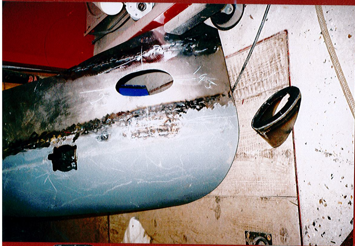
Memo Frenching indicators - Rear Wing Memo NIS Rear Inner wing
