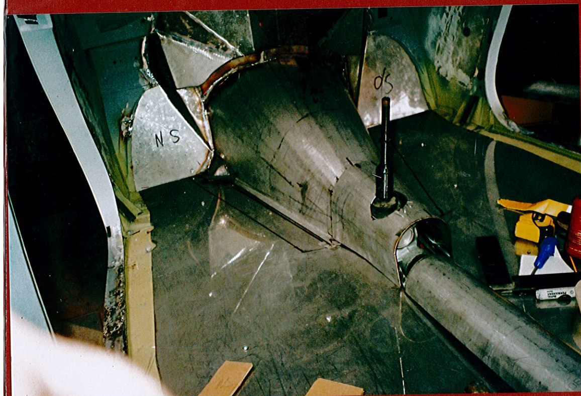
Memo TS Gear box and new prop shaft Memo S/S Transmission tunnel
