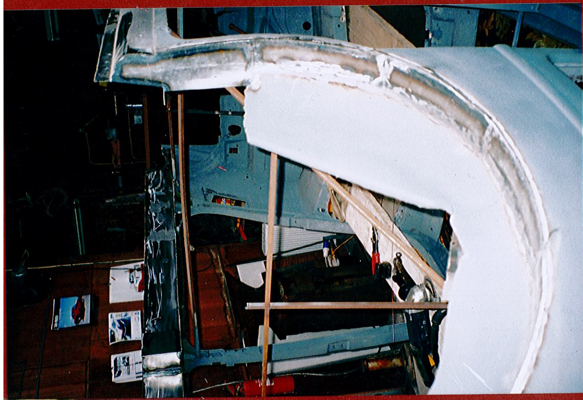
Memo Frenching indicators - Rear Wing Memo NIS Rear Inner wing
