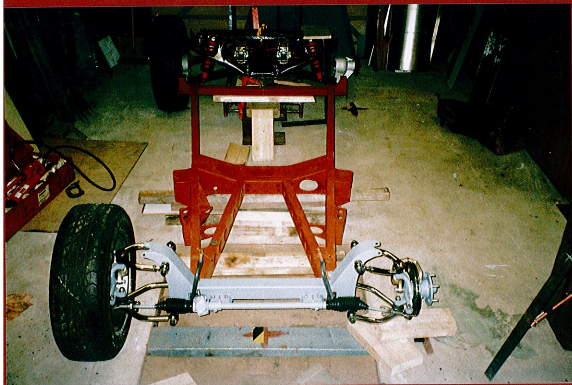
Memo Checking for fit Memo Trill set up of axle
