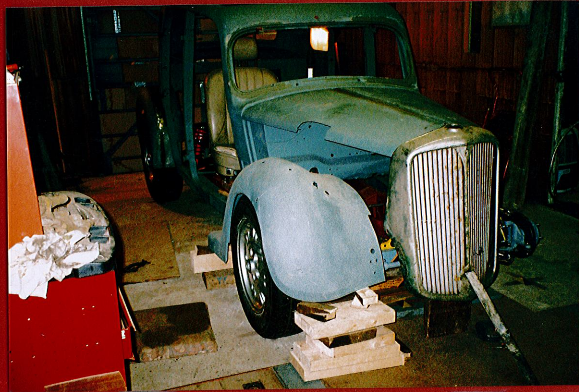
Memo Mock up of front end Memo T.I.E. welding front wing extension.
