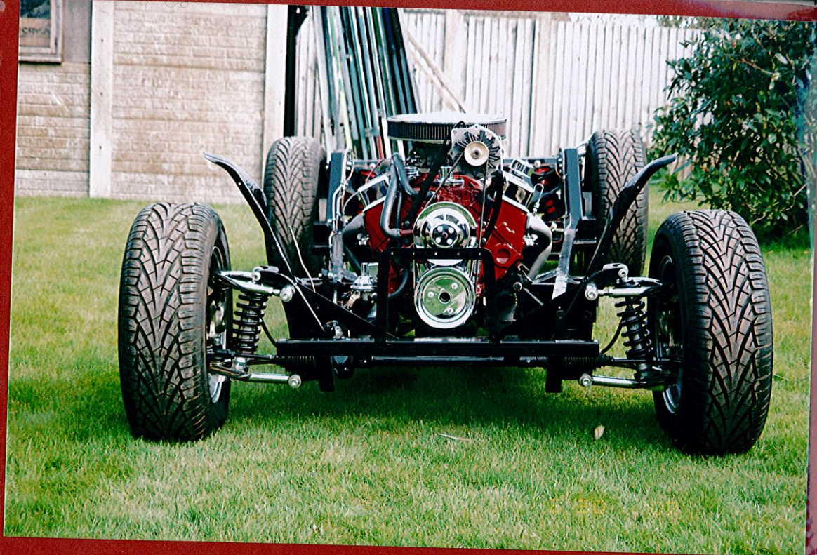
Memo Brake lines in- Memo Fuel lines in. Looking good.
