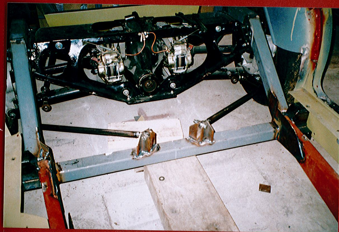
Memo 327 Chevy Engine Memo Rear axle hies fitted
