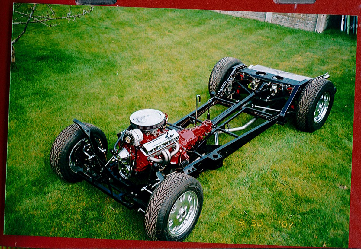
Memo Polishing fuel tank Memo Chassis assembled + plumbed.
