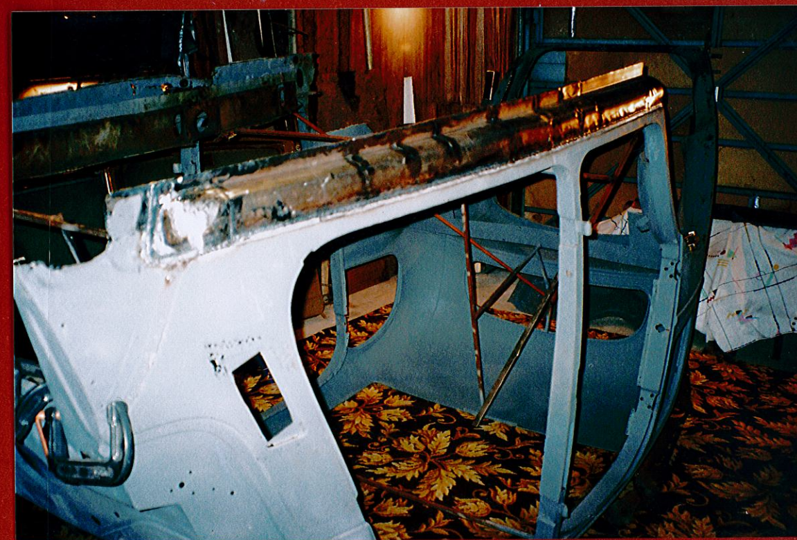
Memo Sill work - OIS Inner complete Memo Outer complete
