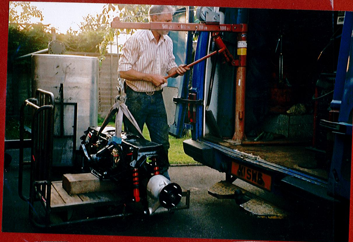
Memo Mark 2 Jag Rear end - rebuilt Memo Wisbech Engineering - front end
